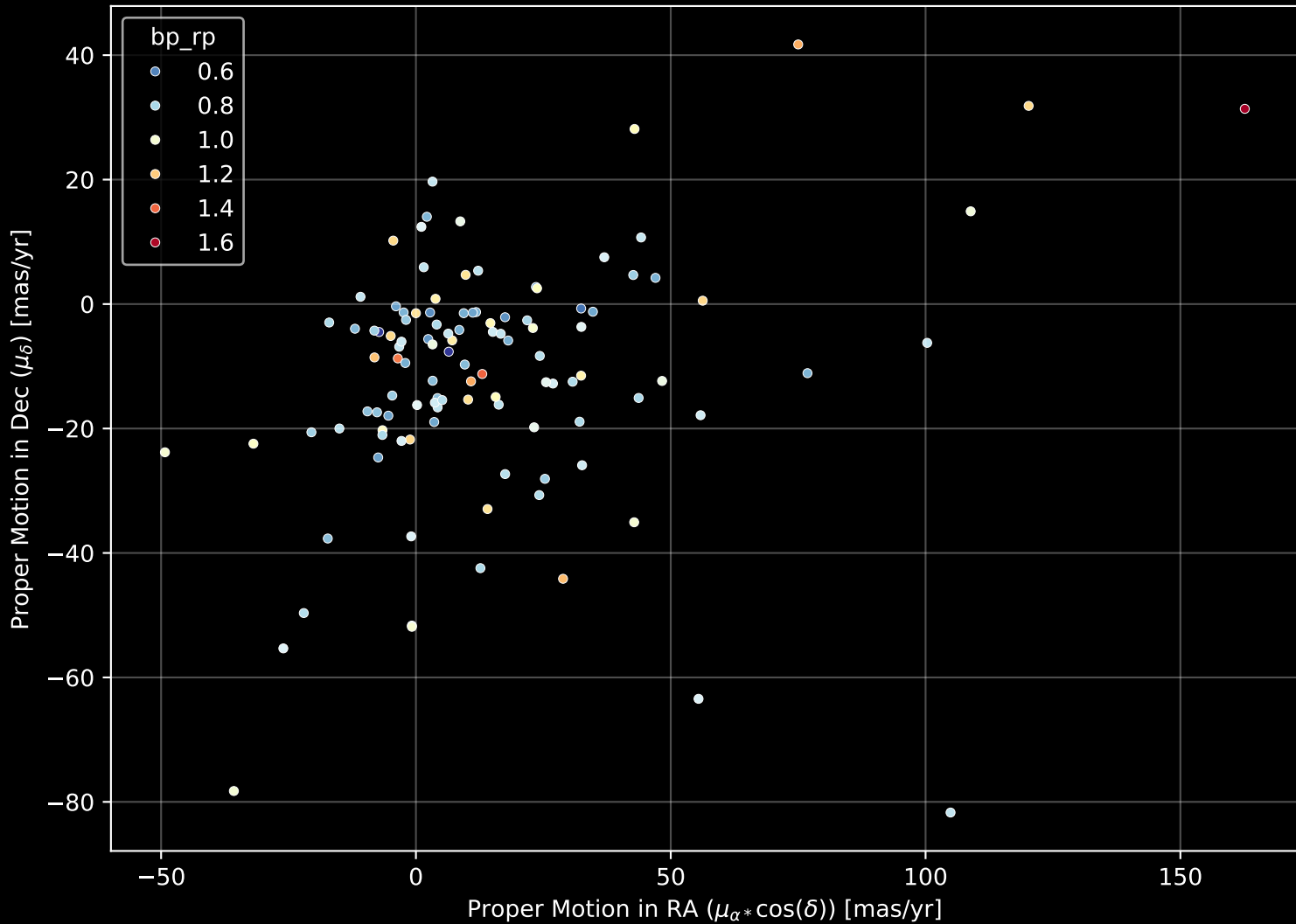
GALAH DR4 Field: [6686] Proper Motion Diagram (n= 112)
