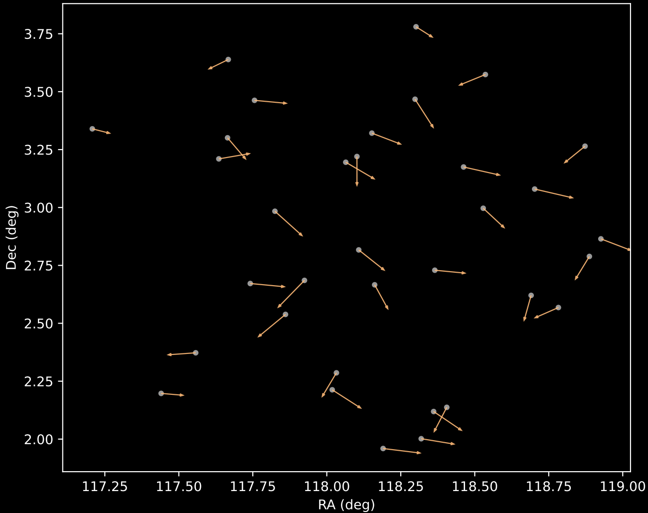
GALAH DR4 Cluster 3 Proper Motion Vectors (n=34)
