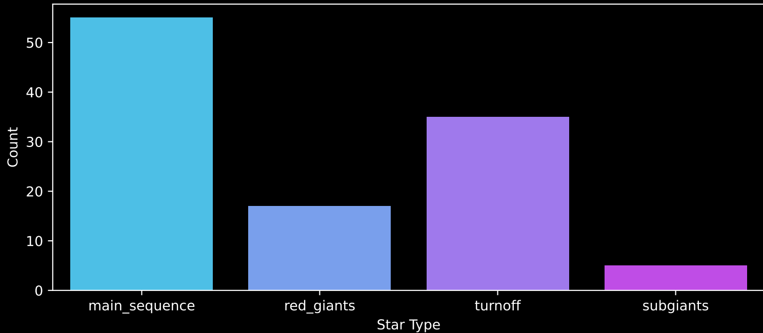
GALAH DR4 Field: [6686] Count plot of Star Type
