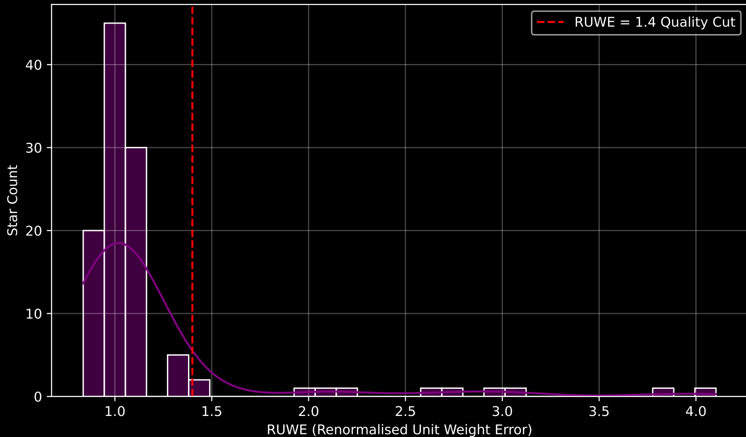
GALAH DR4 Field [6686] RUWE Distribution (n= 111)
